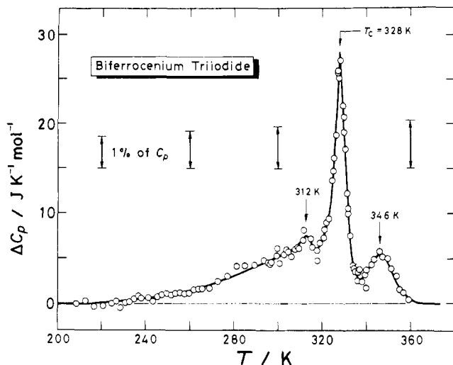
Figure 4. Excess heat capacity, \Delta C_p , due to the phase transition of biferrocenium triiodide.
