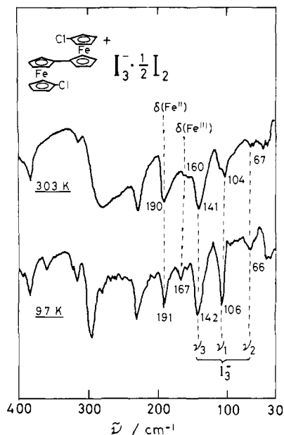
Figure 12. Far-infrared absorption spectra for 1',6'-dichlorobiferrocenium triiodide hemiodine in the range 400–30 cm -1 . \nu_1 , \nu_2 , and \nu_3 indicate the symmetric stretching, deformation, and asymmetric stretching modes of the I_3^- anion. \delta(Fe^{II}) and \delta(Fe^{III}) are the ring-metal-ring bending modes for the Fe^{II} and Fe^{III} metallocene moieties, respectively.
