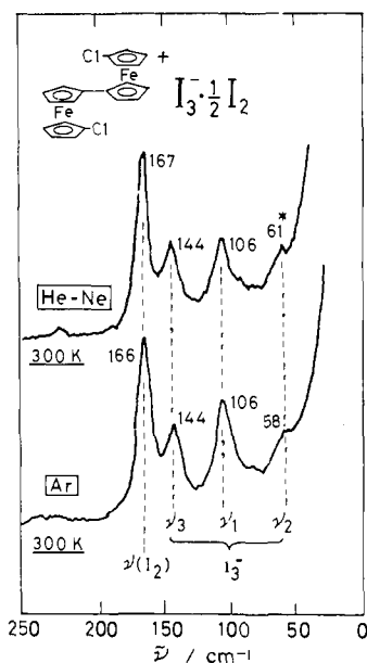
Figure 13. Laser Raman spectra of 1',6'-dichlorobiferrocenium triiodide hemiodine in the range 250–40 cm -1 , recorded by using either a He-Ne or an Ar source. See the caption for Figure 12 for a definition of \nu_1 , \nu_2 , and \nu_3 .
