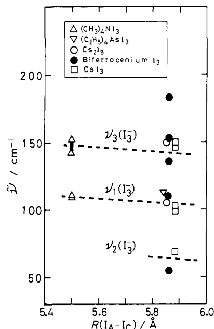
Figure 11. Dependence of the \nu_1 , \nu_2 , and \nu_3 fundamental modes of vibration in I_3^- ion upon the bond length between the two terminal atoms of the triiodide anion for various compounds. For biferrocenium triiodide, all the bands observed in IR and Raman spectra below 200 cm^{-1} are plotted.
