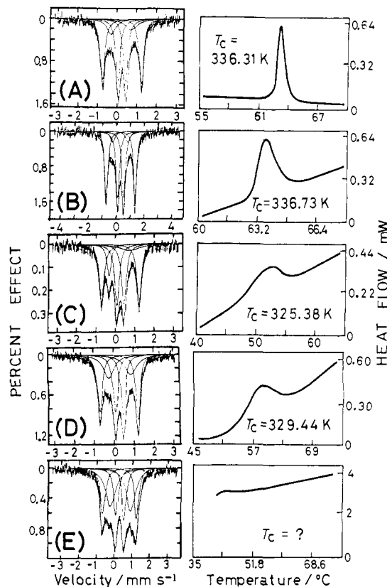
Figure 5. Sample history dependence of the ^{57}\text{Fe} Mössbauer spectrum at 300 K and DSC thermogram for biferrocenium triiodide. Samples A and B are two different microcrystalline samples that were prepared in the same manner. Sample C is comprised of recrystallized well-grown crystals. Samples D and E correspond to specimens taken from the two batches used for the heat capacity measurement. The DSC thermograms were run at a scan rate of 10 deg/min.
